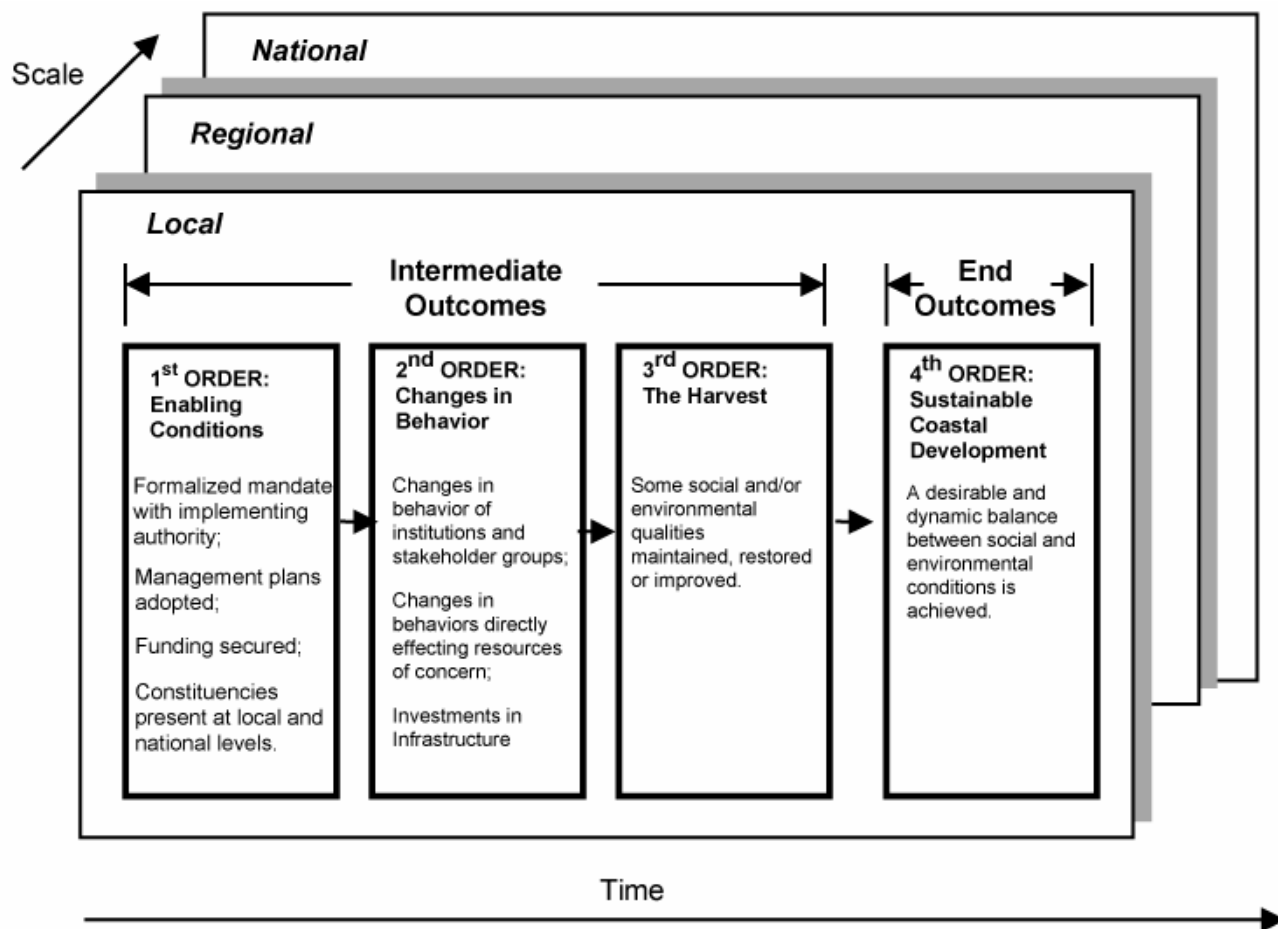
Fig. 1. The four orders of coastal governance outcomes.
